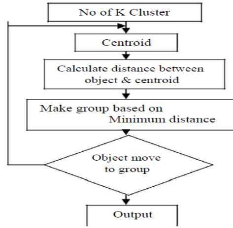
Fig-1 K-means algorithm.
